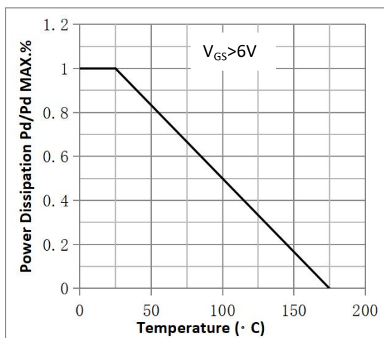
Fig.3 Power Dissipation
