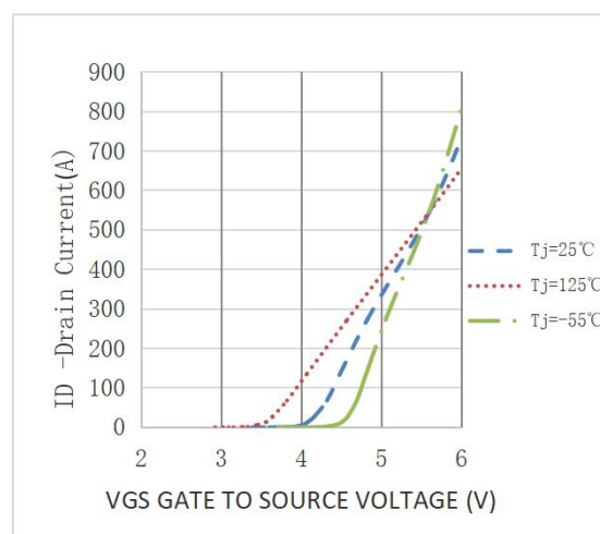
Figure 10. Transfer Characteristics
